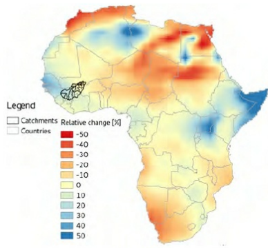
(a) GFDL
