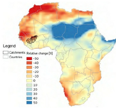
(b) HadGEM
