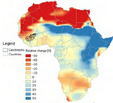
(c) IPSL
